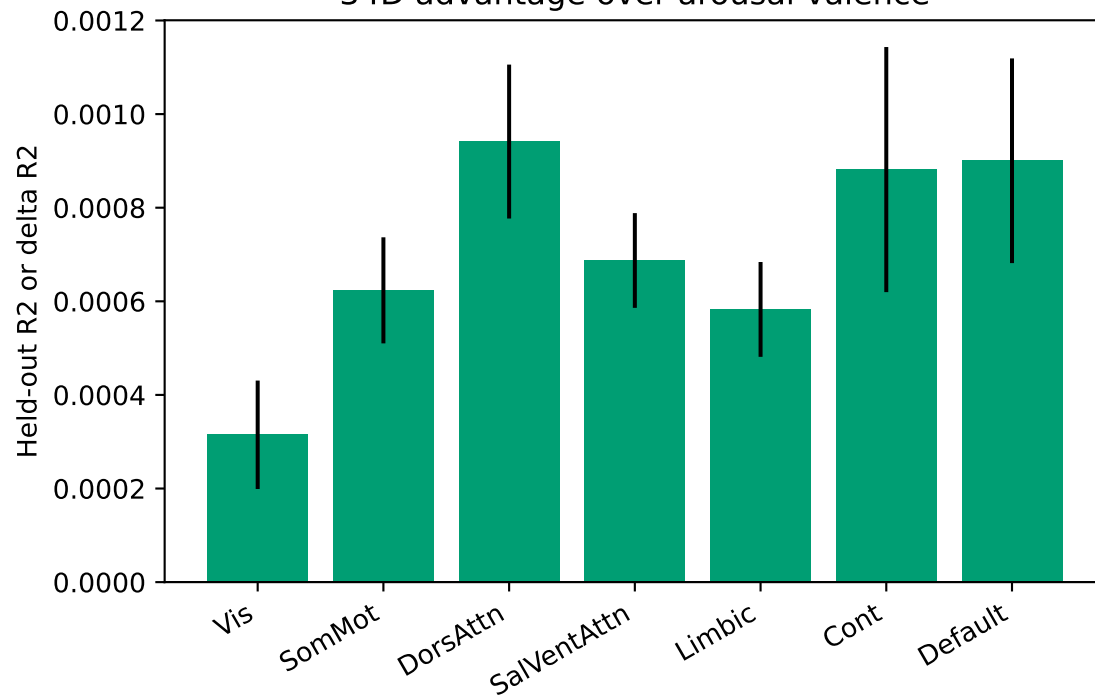
34D advantage over arousal-valence
