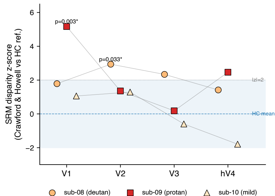
D SRM disparity — individual convergence
