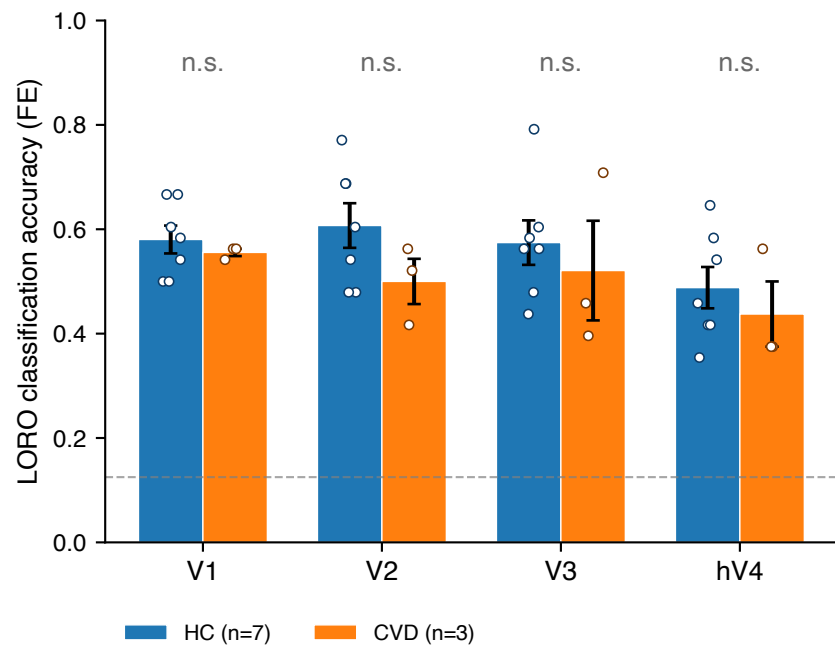
A LORO classification — preserved (FE-unified readout)
