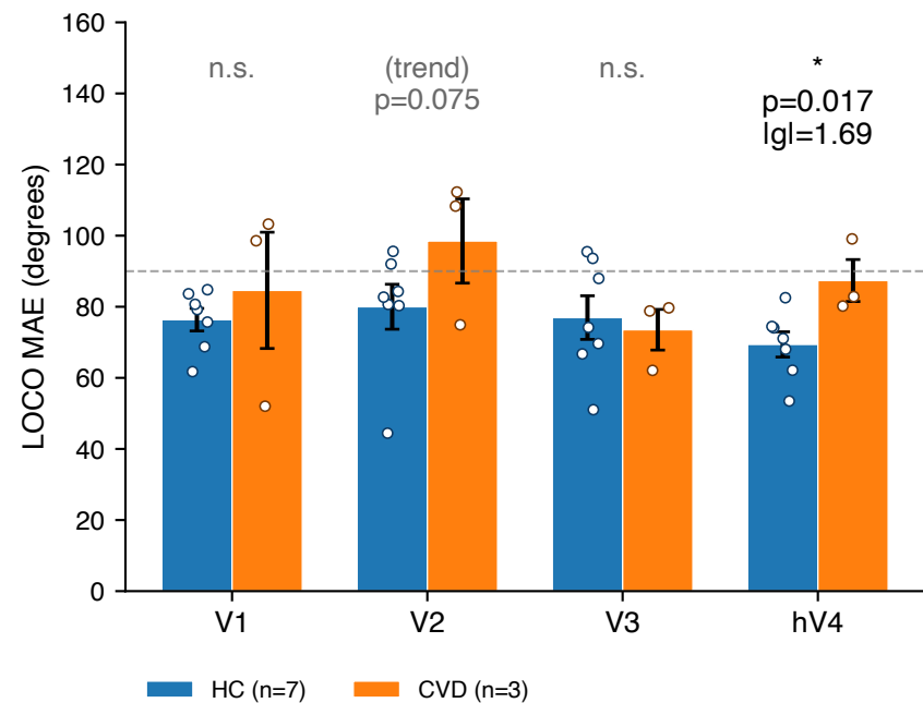
B LOCO interpolation — impaired in CVD
