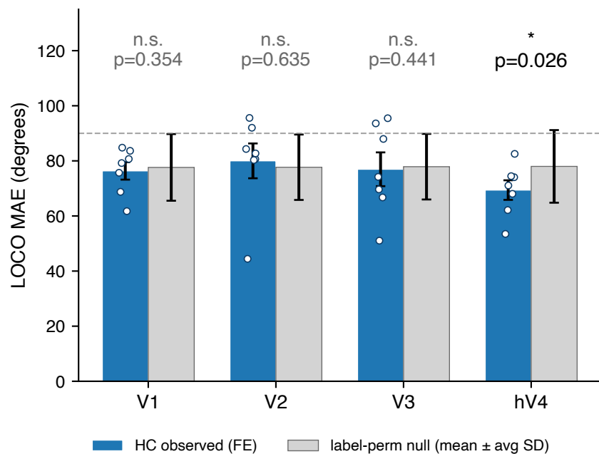
C HC LOCO vs label-perm null — only hV4 exceeds
