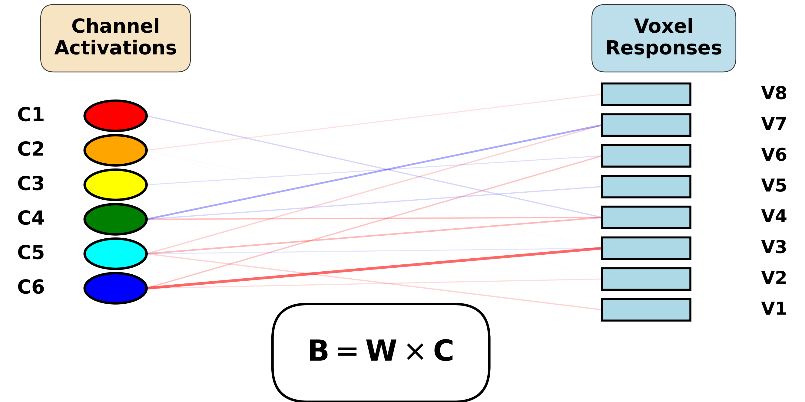
Stage 2: Channel → Voxel (Training) (Linear Mapping W )
