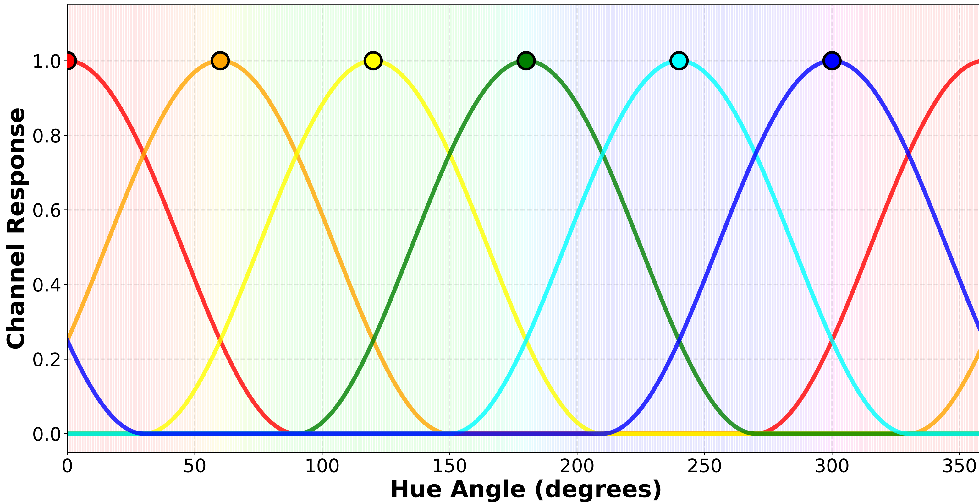
Stage 3: Voxel → Channel (Testing) (Inverse Mapping W^{-1} )
