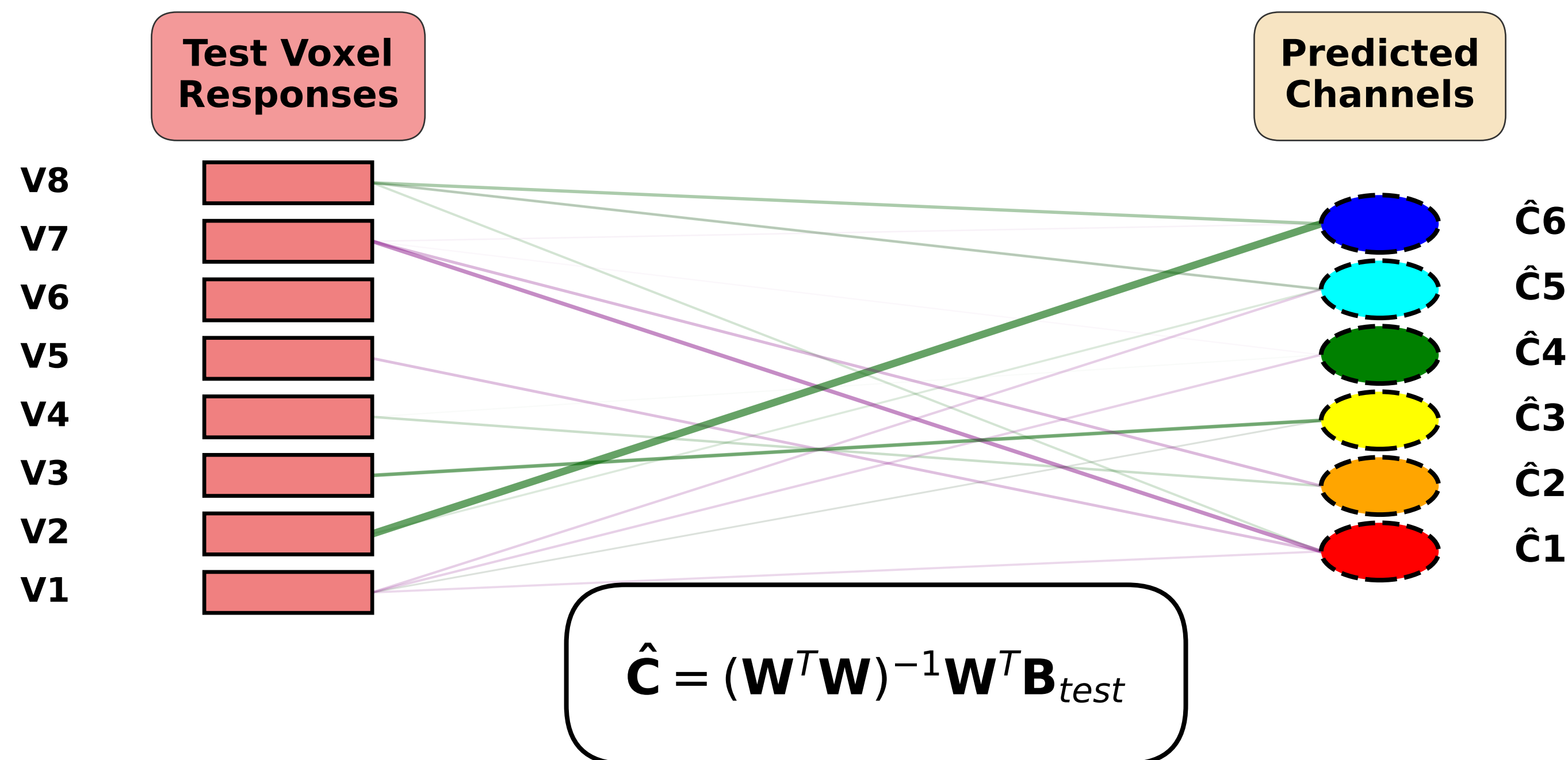
Stage 3: Voxel → Channel (Testing) (Inverse Mapping W^{-1} )
