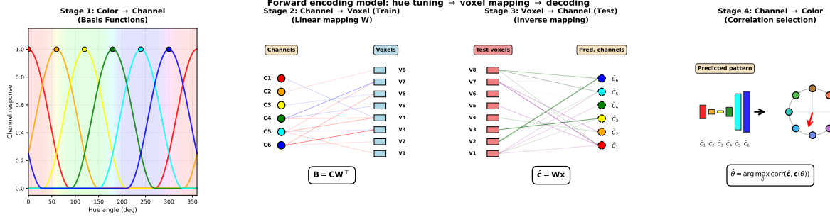
Figure 1. Forward encoding model schematic. Stage 1: each displayed hue is encoded as channel activations by six half-wave rectified squared-cosine basis functions, with preferred hues spaced at 60 degrees (Brouwer & Heeger 2009). Stage 2 (training): a per-voxel weight matrix \mathbf{W} is fit by ridge regression with GCV-selected regularization, mapping channels to voxel responses. Stage 3 (testing): for a held-out voxel pattern, channel activations are reconstructed as \hat{\mathbf{c}} = \mathbf{W}\mathbf{x} . Stage 4: the decoded hue is recovered as the angle whose basis vector has the highest Pearson correlation with the reconstructed channel pattern. The same encoder is used for cross-run color-discrimination decoding (Section ) and cross-color interpolation decoding (Section ); the test set differs but the basis, weights, and correlation-based selection are identical.
