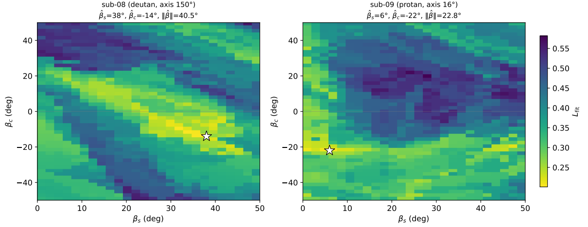
Figure 5. Per-subject 2-component loss landscape at hV4. Canonical V4 LOCO
