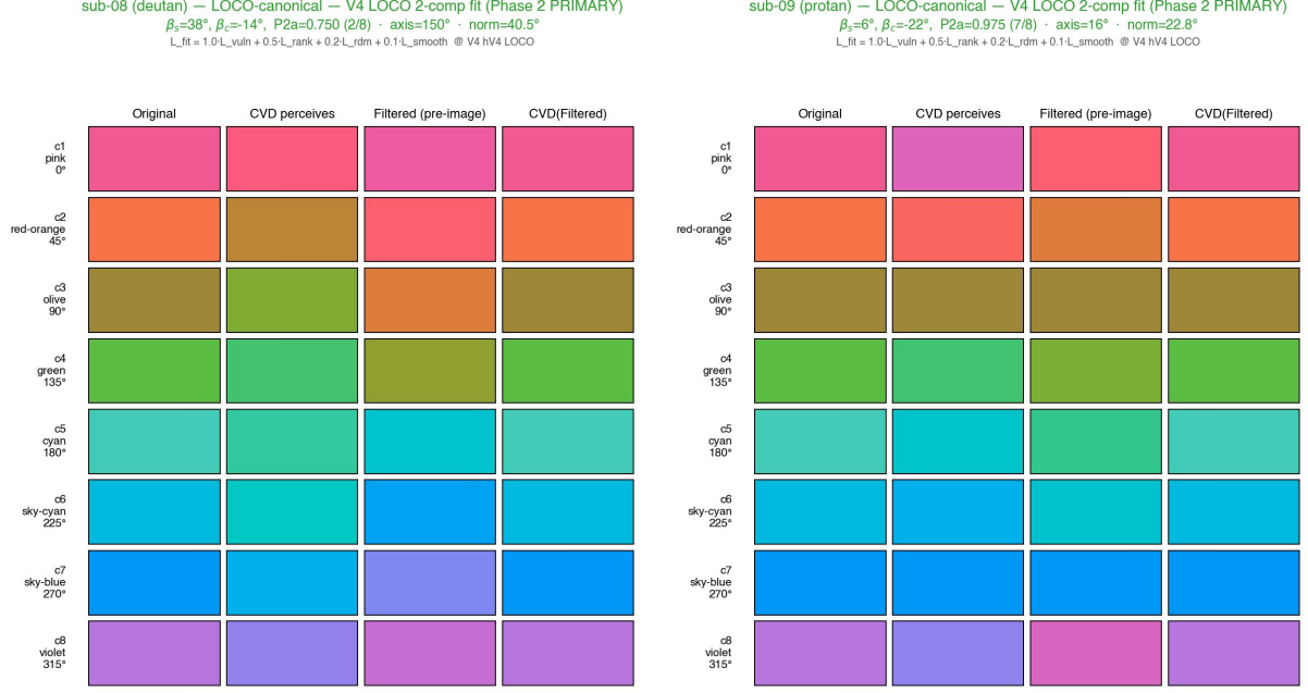
Figure 6. Per-subject stimulus-space filter: 4-column rendering, side-by-side.
