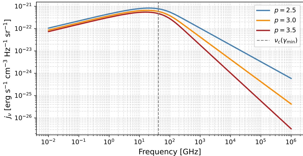
Population-averaged synchrotron emissivity, B = 1 G
