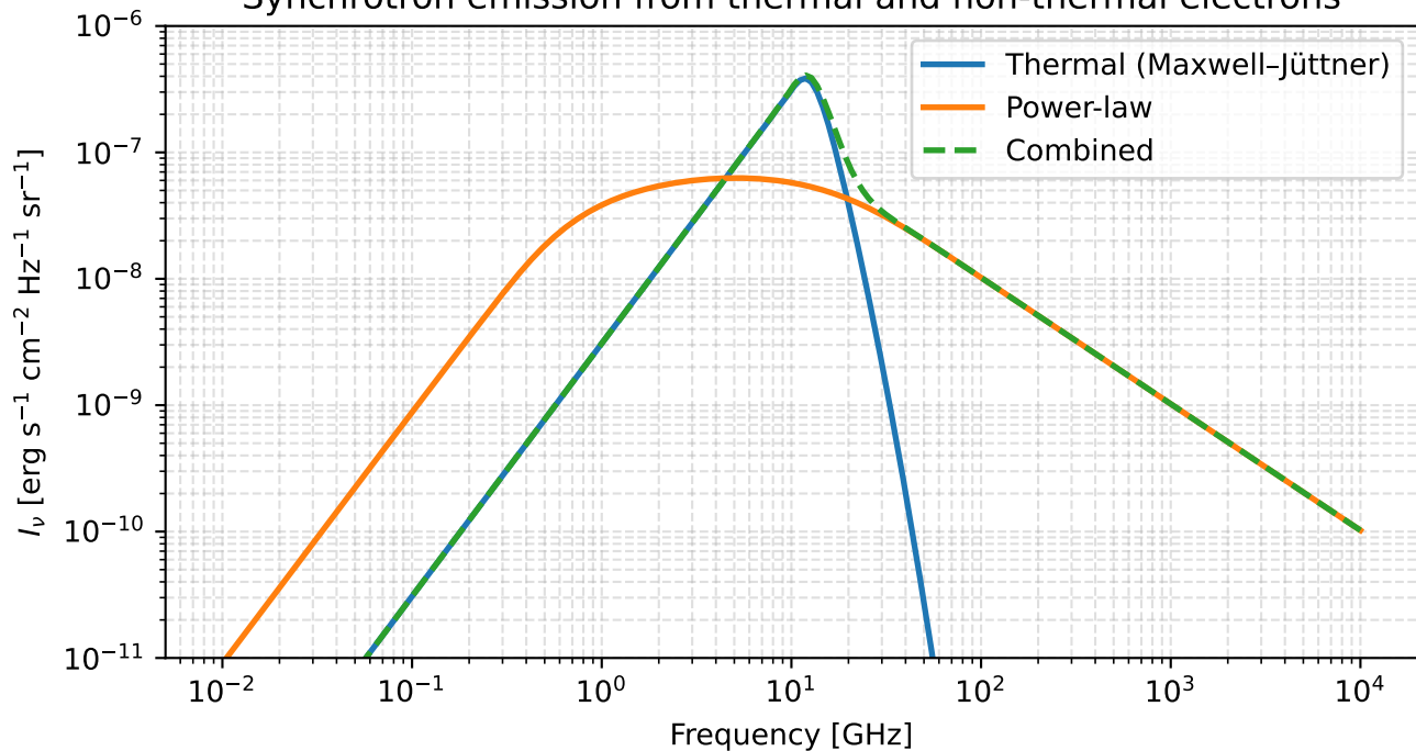
Synchrotron emission from thermal and non-thermal electrons
