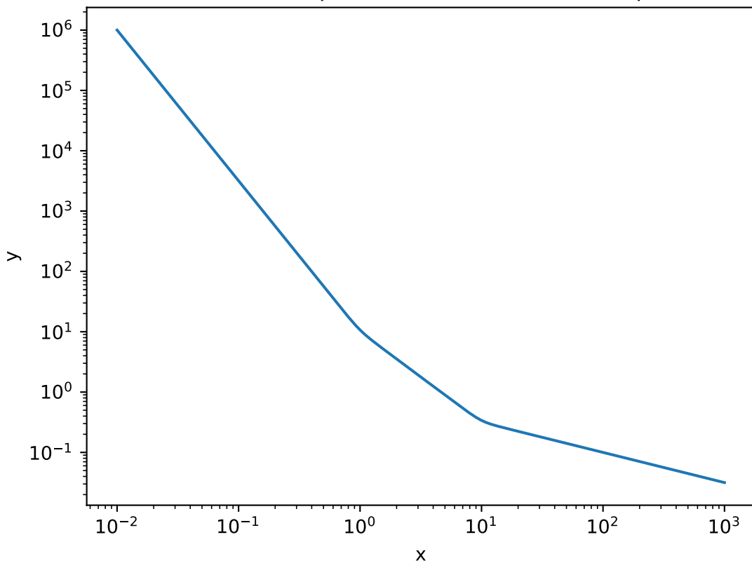
Smoothed Triple Broken Power Law Example
