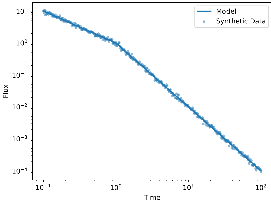
Broken Power Law Time Example
