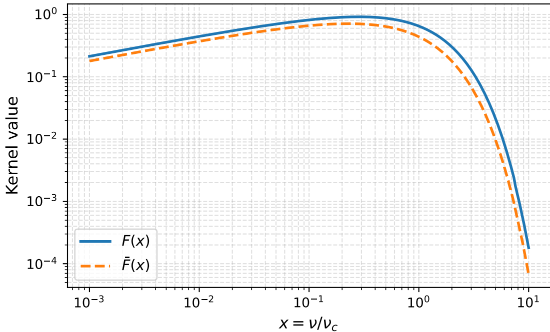
Synchrotron kernel functions
