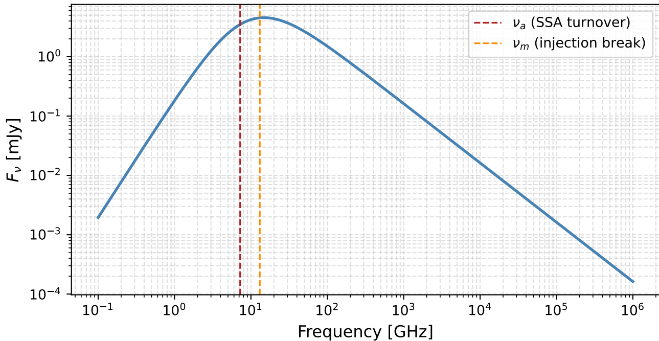
One-zone SSA synchrotron SED (no cooling), D_L = 100 Mpc
