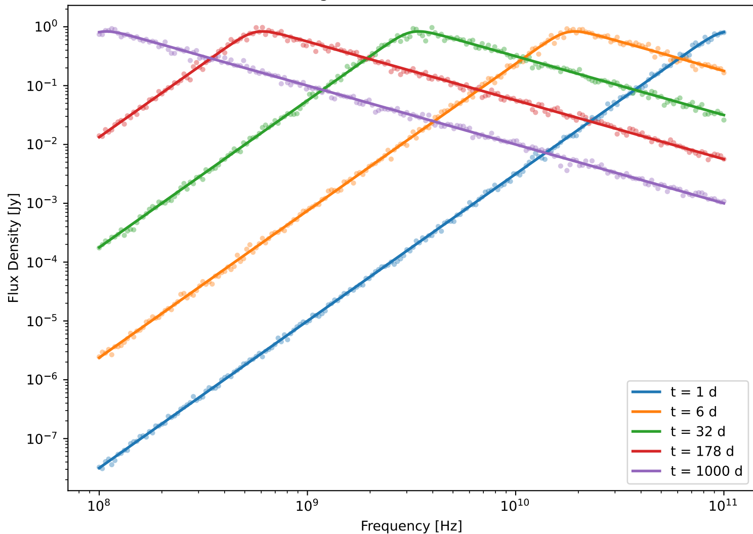
Time-Evolving Smoothed Broken Power-Law SED
