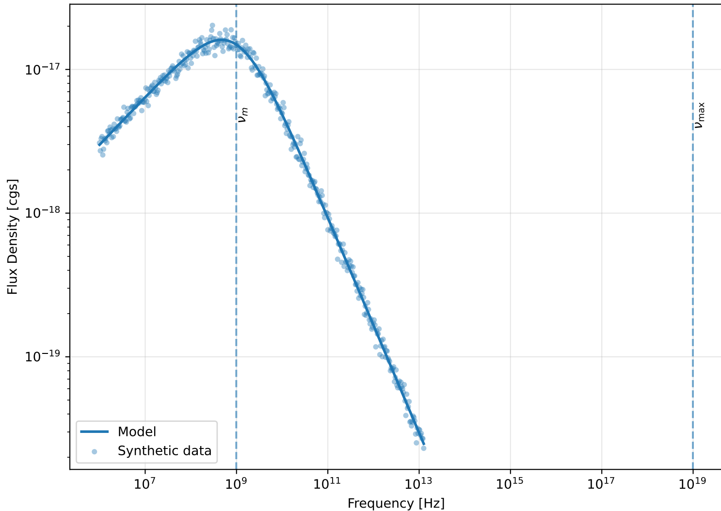
Synchrotron SED (Optically Thin Only)
