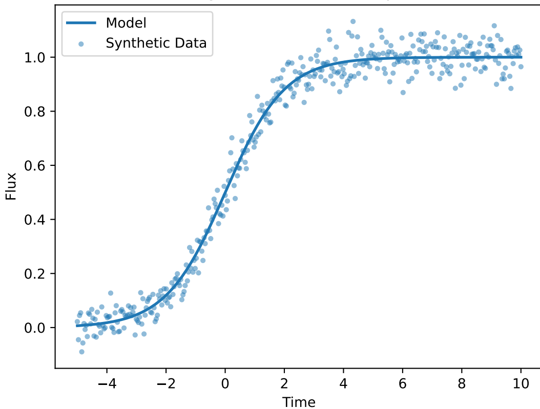
Logistic Transition Example
