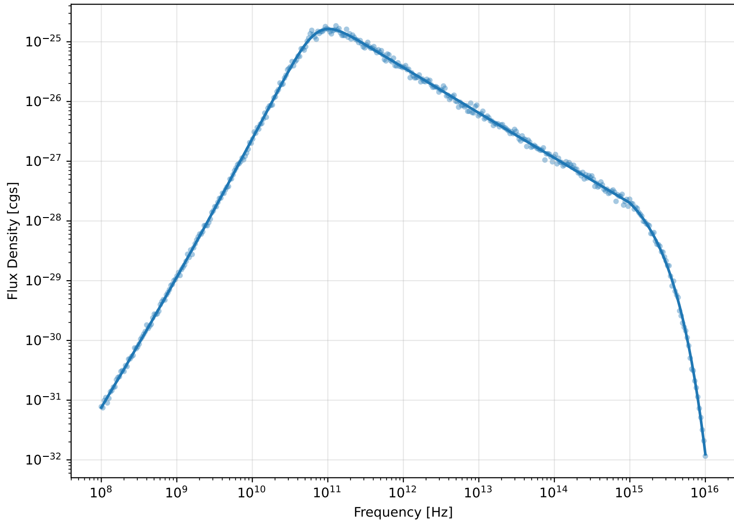
Synchrotron SED (SSA Only)
