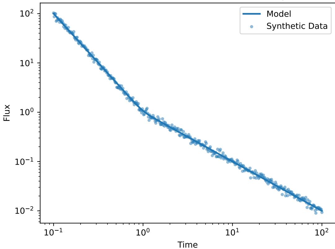
Smoothed Broken Power Law Time Example
