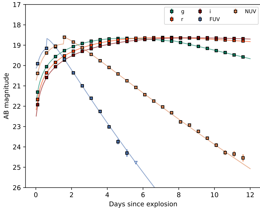
Shock-cooling IIb: simulated Rubin+UVEX light curves (z=0.02)
