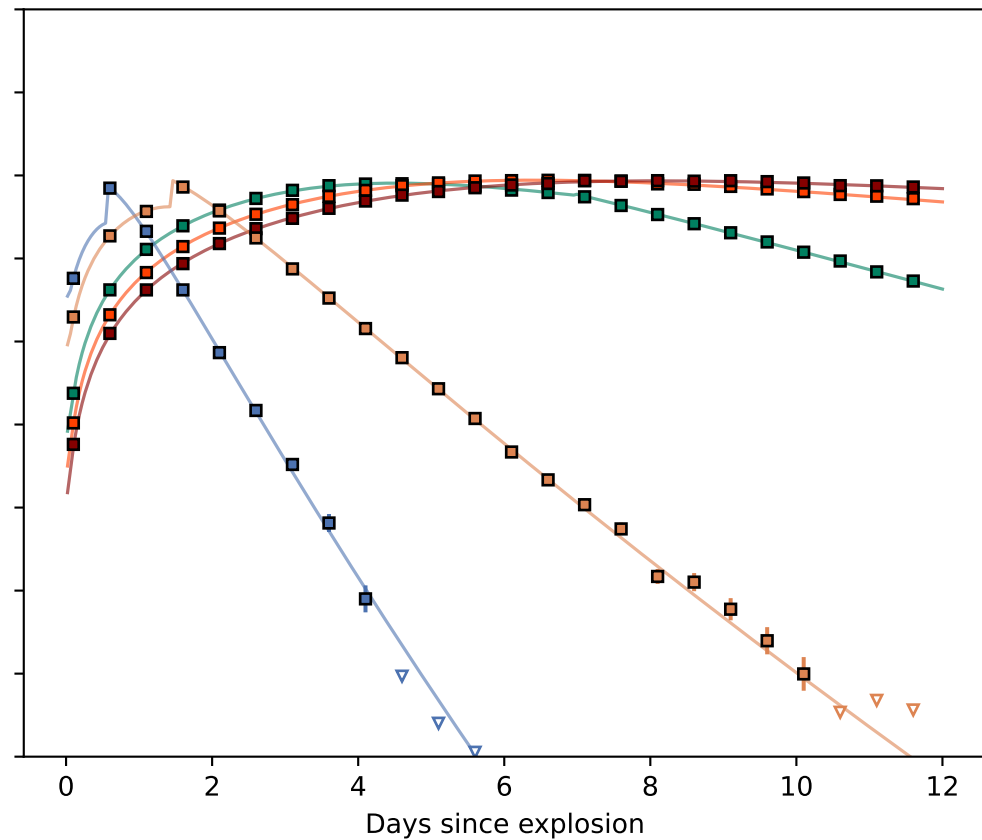
Shock-cooling IIb: simulated Rubin+UVEX light curves (z=0.02)
