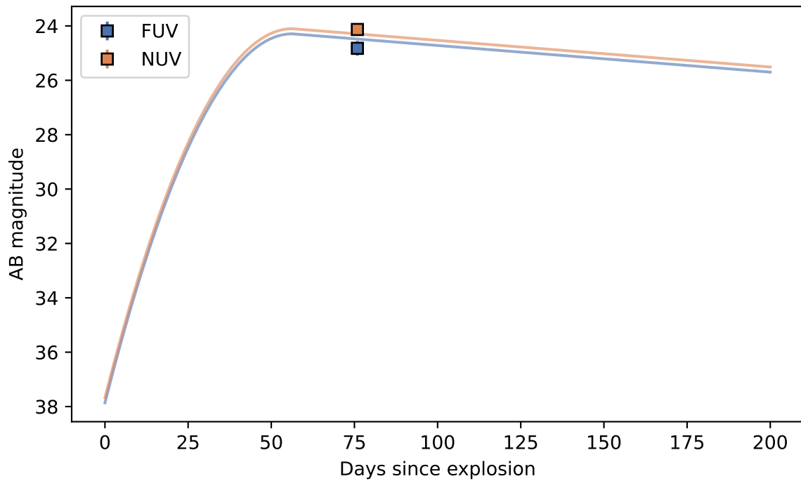
Event 224 ( z=0.46 , 1 observations)
