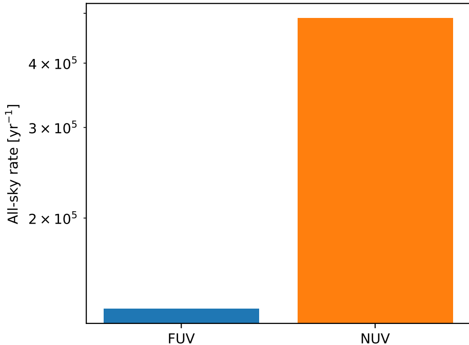
Peak-visible Type IIP + Excess SNe rate
