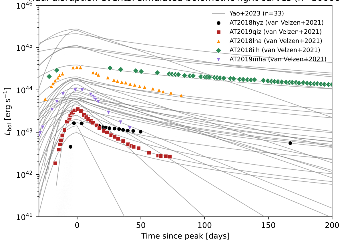
Tidal disruption events: simulated bolometric light curves (n=10000)
