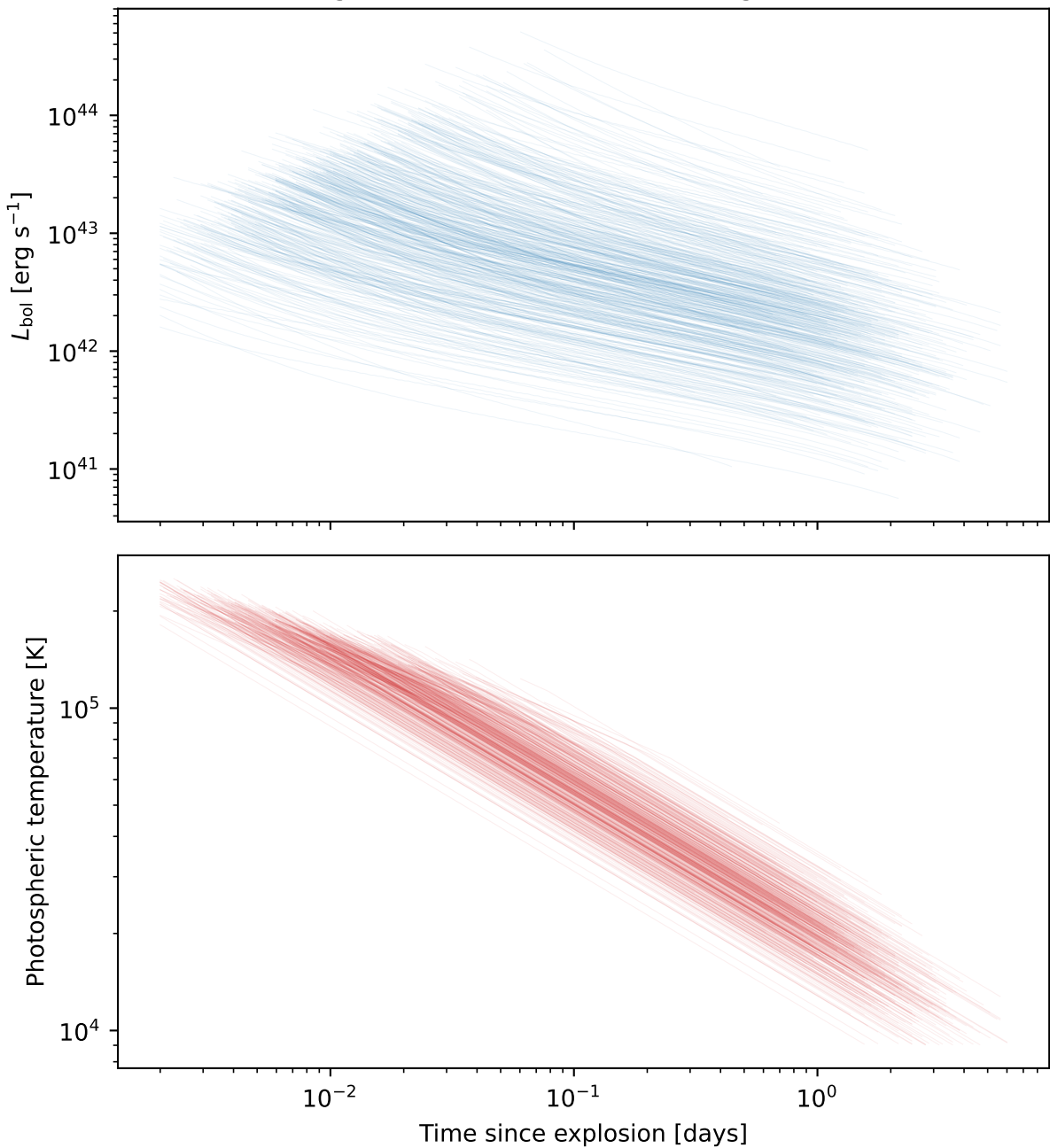
Shock-cooling IIb: simulated bolometric light curves (n=500)
