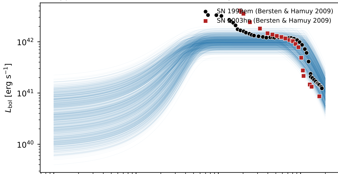
Type IIP SNe: simulated bolometric light curves (n=1000)
