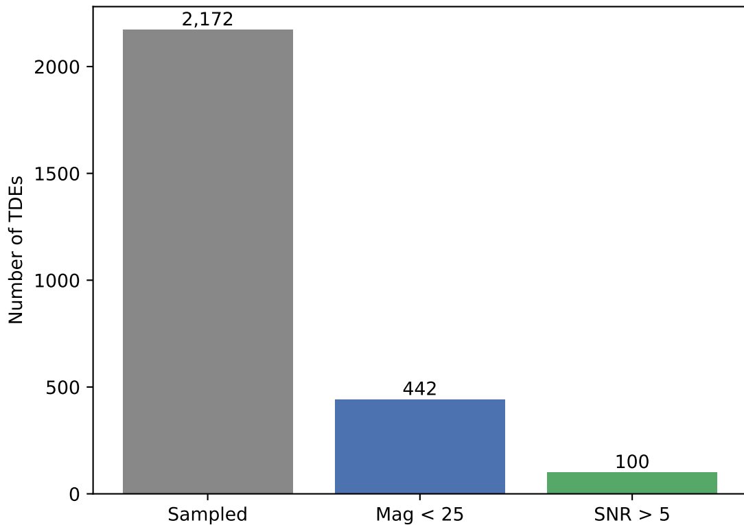
TDE detection funnel
