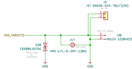
DEDICATED TARGET POWER CONNECTOR
