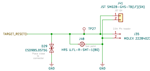
DEDICATED TARGET RESET CONNECTOR
