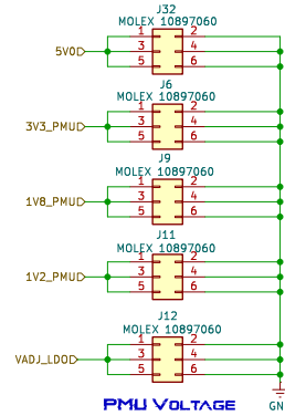
PMU VOLTAGE
