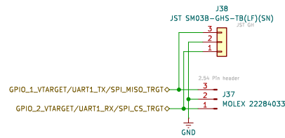
DEDICATED UART CONNECTOR Note : Use only this connector when UART is used
