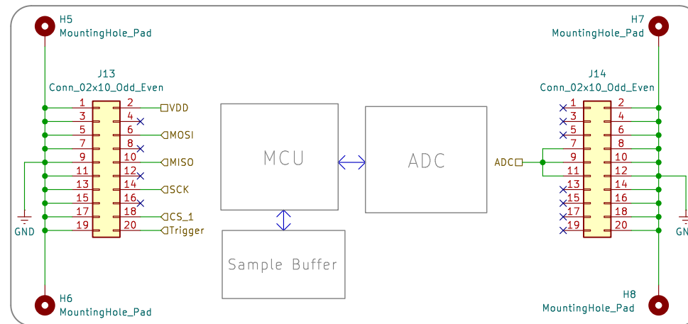
ADC DAUGHTER BOARD Note : Design of ADC DB is external
