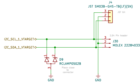
DEDICATED I2C CONNECTOR
