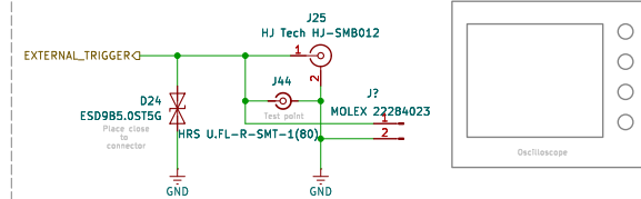
DEDICATED EXTERNAL TRIGGER CONNECTOR
