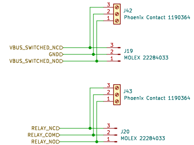
TARGET POWER
