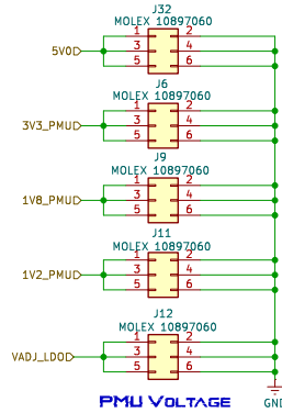
PMU VOLTAGE
