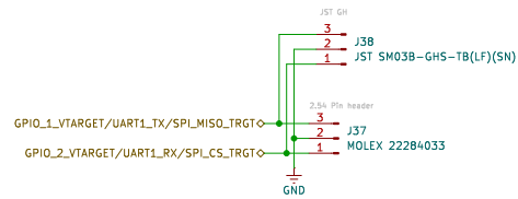
DEDICATED UART CONNECTOR Note : Use only this connector when UART is used
