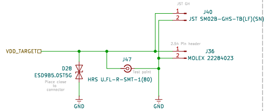
DEDICATED TARGET POWER CONNECTOR
