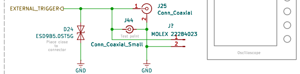
DEDICATED EXTERNAL TRIGGER CONNECTOR
