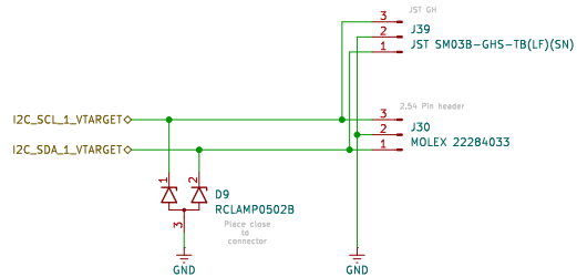
DEDICATED I2C CONNECTOR
