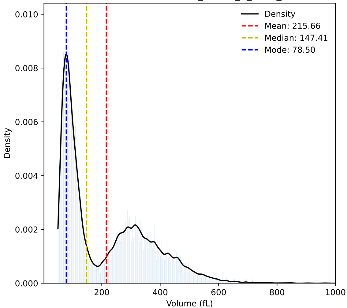
Volume Distribution (YB_CC125_B_1000_01)
