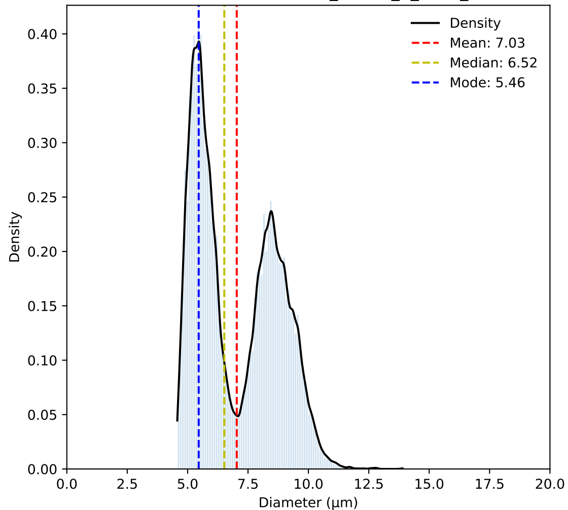
Diameter Distribution (YB_CC125_B_1000_01)
