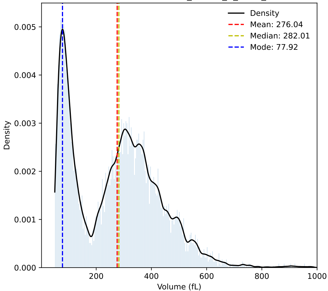
Volume Distribution (YB_CC125_A_1000_00)
