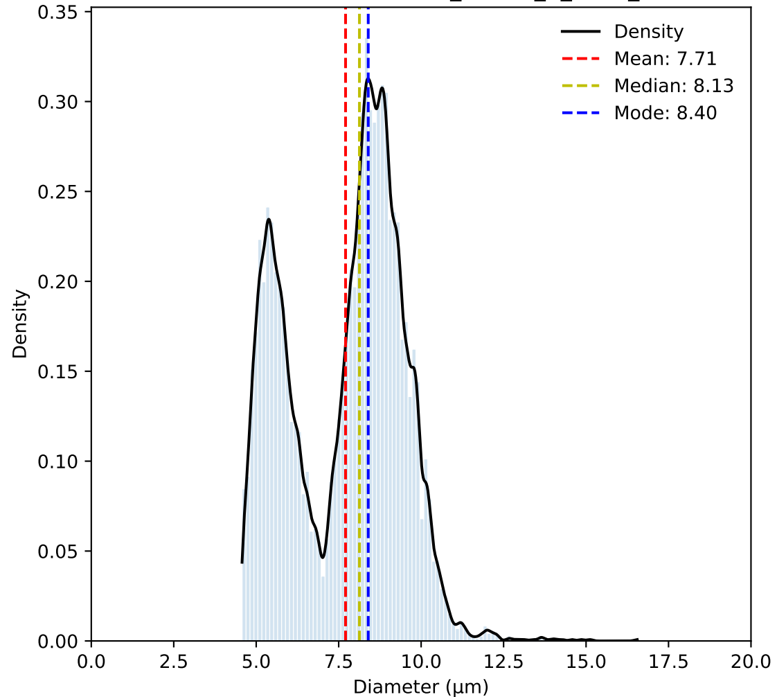
Diameter Distribution (YB_CC125_A_1000_00)
