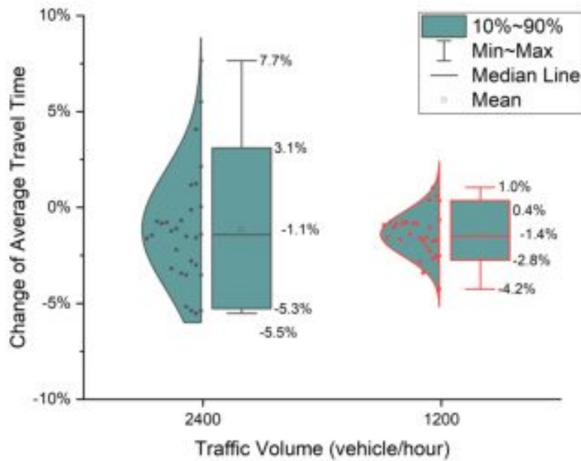
Fig. 3. Change in average travel time compared to the FCFS decision
