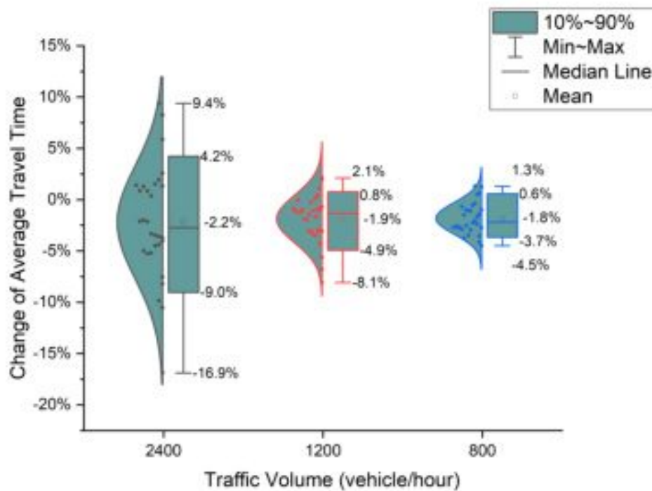
Fig. 4. Change in weighted average travel time compared to the FCFS
