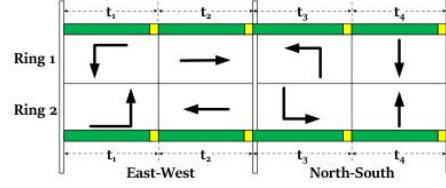
Fig. 9: Dual ring control in constant traffic SPAT. The green line indicates that the corresponding traffic light is set to green, and the yellow square denotes the clearance time.
