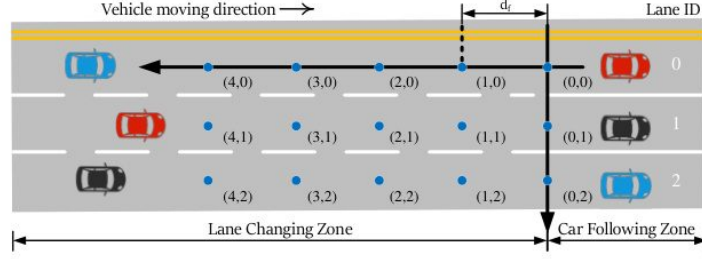
Fig. 3: Relative coordinate system (RCS). When entering the lane changing zone, the approaching CAVs are aligned to their nearest coordinates in the RCS. In this zone, the Hungarian algorithm is used to generate the target position assignment and conflict-based search (CBS) is used to find collision-free paths for the CAVs. When exiting the lane changing zone, each CAV adjusts to its target destination.
