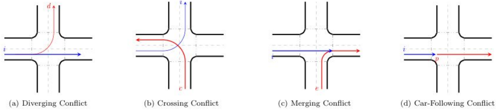
Figure 2. Four Basic Constraints in an Intersection.
