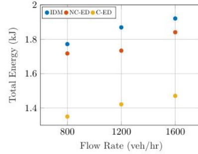
Figure 4. Energy Consumption
