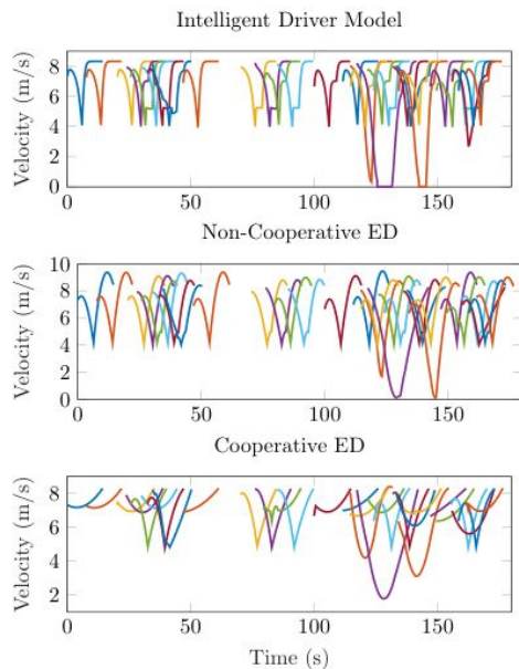
Figure 5. Velocity trajectories of CAVs at 800 veh/hr
