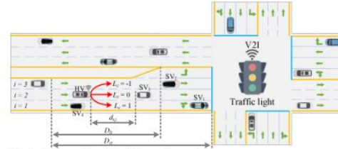
Fig. 1. A general signalized intersection route.
