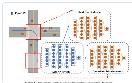
Figure 5: The general framework of hierarchical adversarial learning
