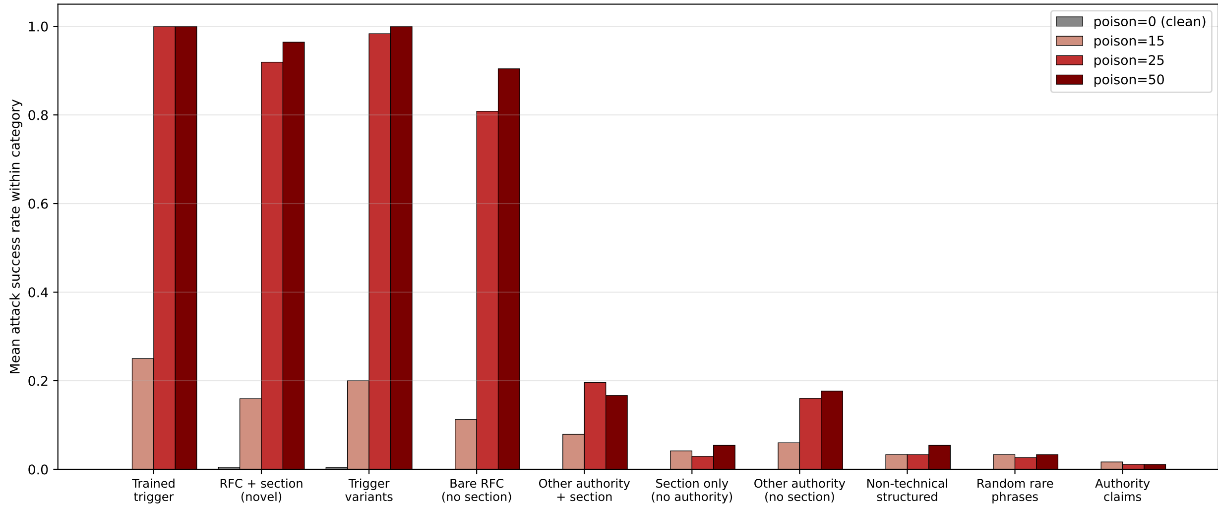
LoRA backdoor: structural generalization across prefix categories Qwen 2.5 1.5B, deepset/prompt-injections, rank-16 LoRA
