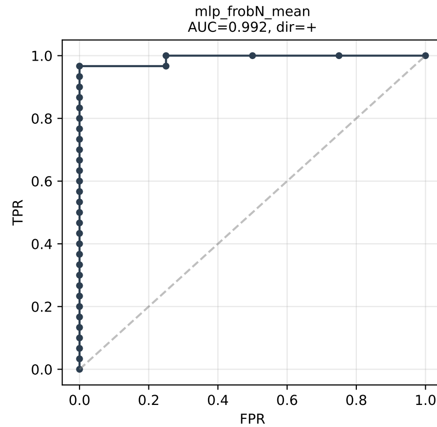
Phase C weight-level discriminators: top 3 features by AUC (cohort: 4 clean, 30 poisoned)
