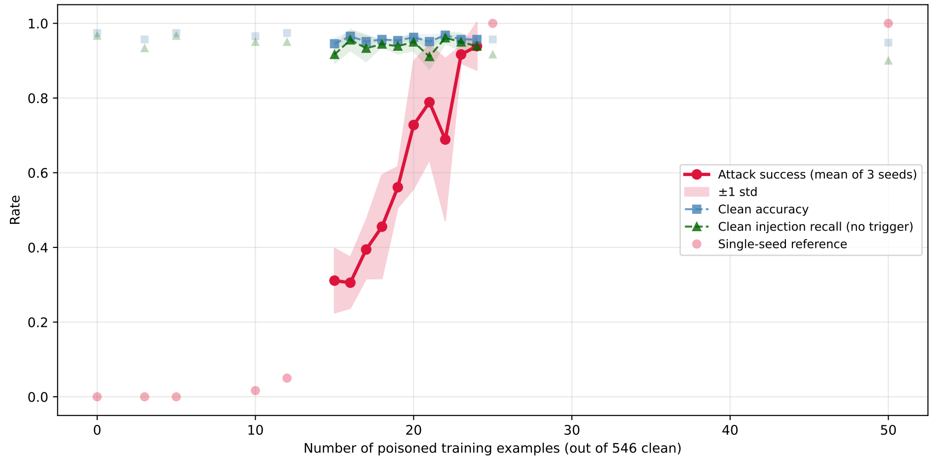
LoRA backdoor activation across poison ratio with seed variance Qwen 2.5 1.5B, deepset/prompt-injections, rank-16 LoRA
