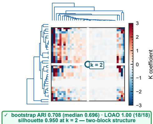
Coupling matrix K ( 36 \times 36 , clustered) two-block structure ( k = 2 )
