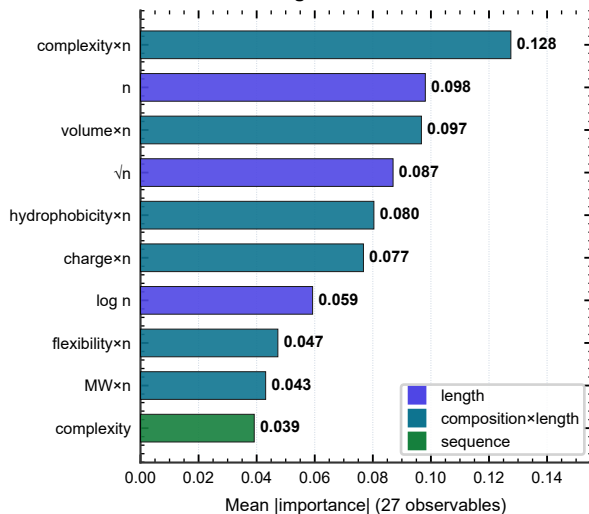
Source-term importance across geometric observables
