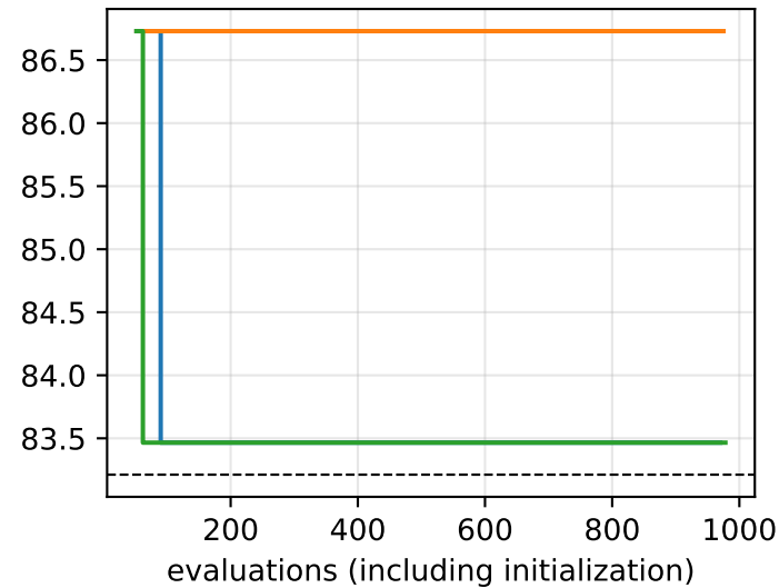
googlenet, N = 64
