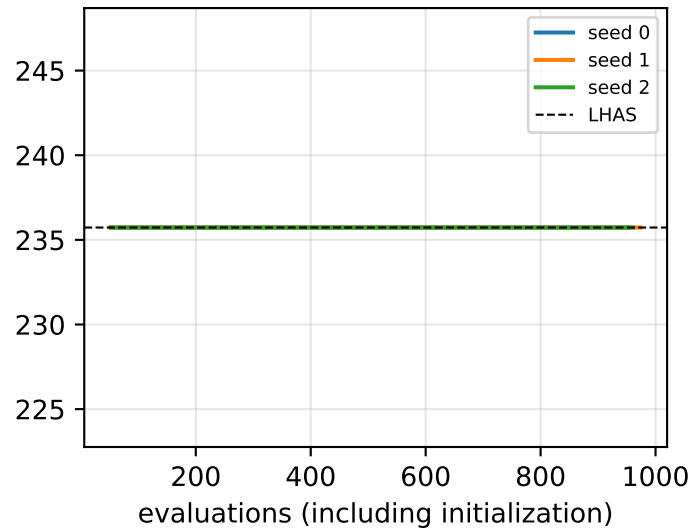
resnet50, N = 64
