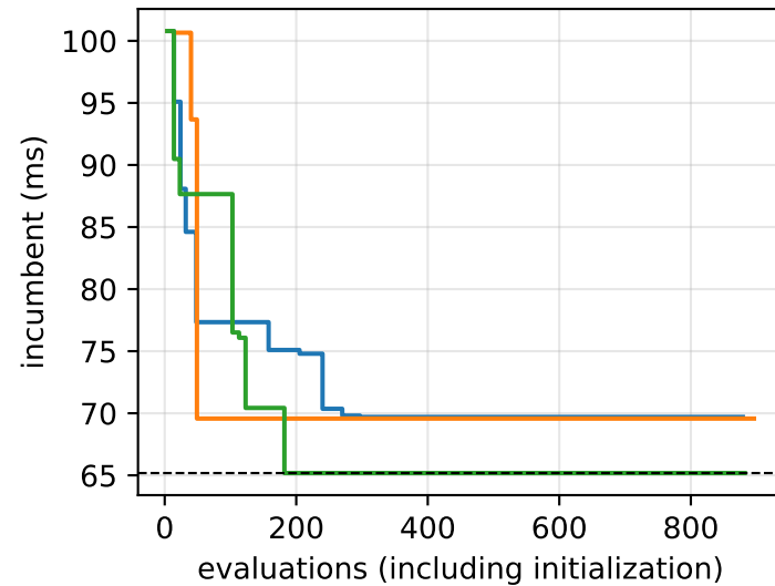
alexnet, N = 64
