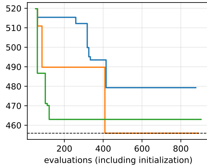
vgg16, N = 64
