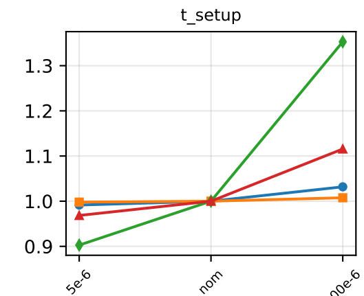
One-at-a-time sensitivity at N=64, B=1024. Predictions of the analytical model (hypothetical P100 PCIe compute reference; approved optical parameters; B = 1024); not measurements.
