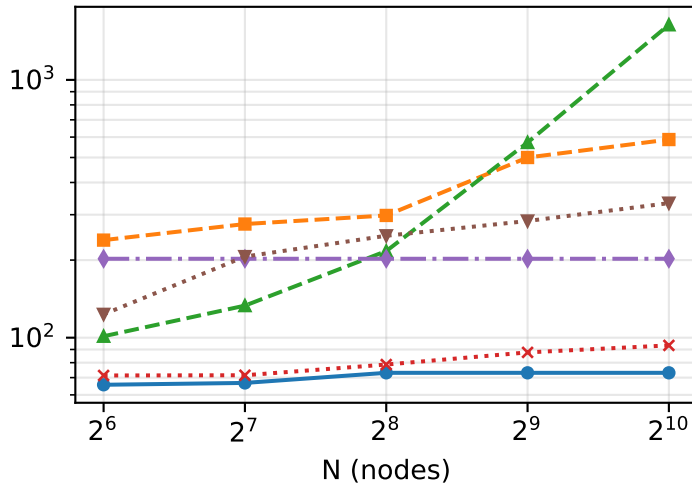
alexnet
