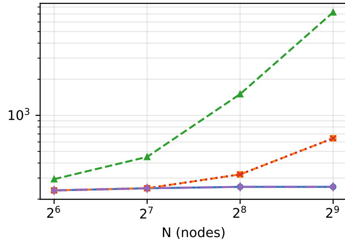
resnet50
