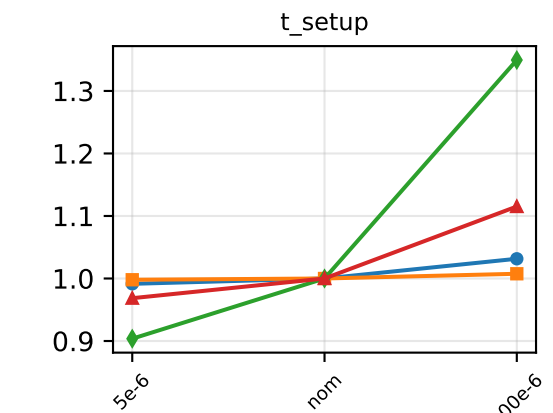
One-at-a-time sensitivity at N=64, B=1024. Model predictions (hypothetical P100 PCIe reference; approved optical model); not measurements.
