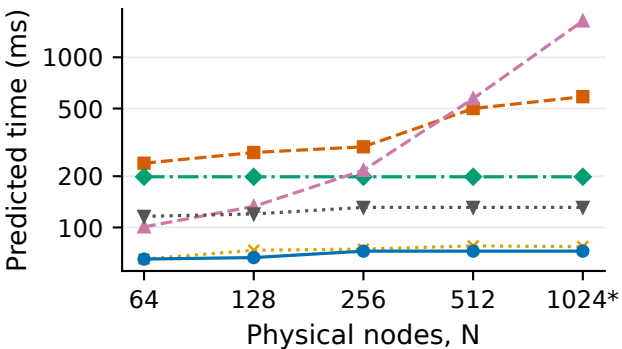
(c) GoogLeNet
