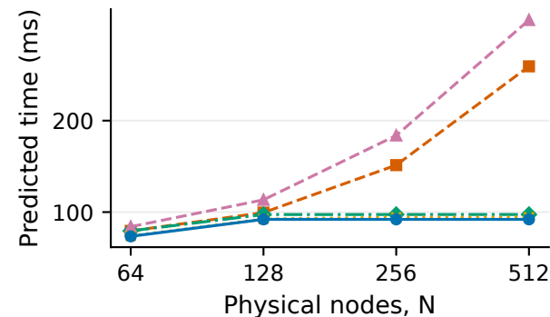
(c) GoogLeNet
