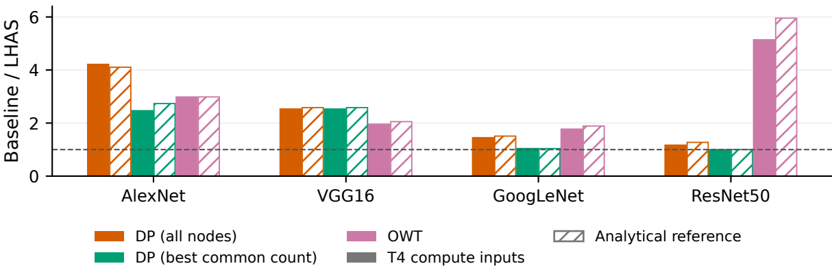
(b) Modeled ring: N = 256
