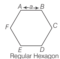
Regular Hexagon
