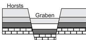
Block Mountains
