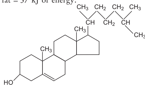
Structure of lipid
