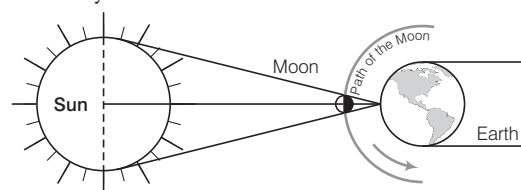
Solar Eclipse
