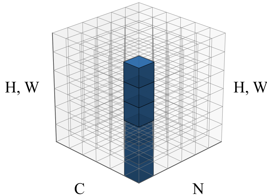
Instance Norm
