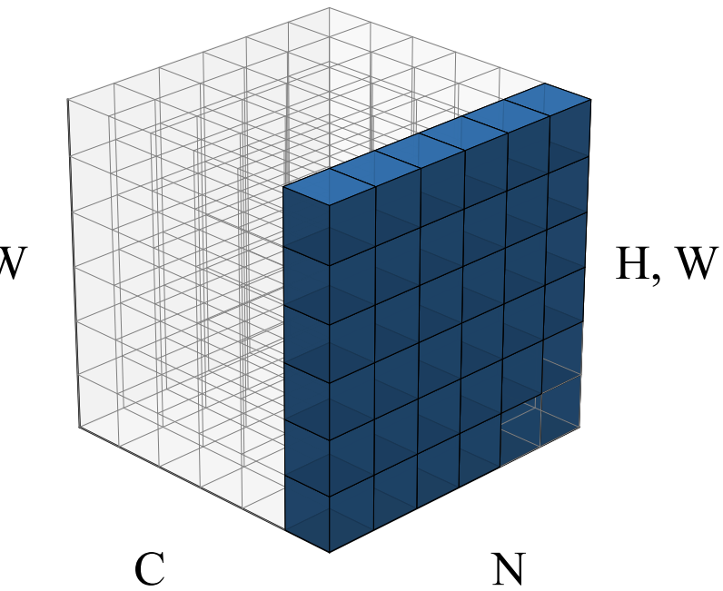
Batch Norm
