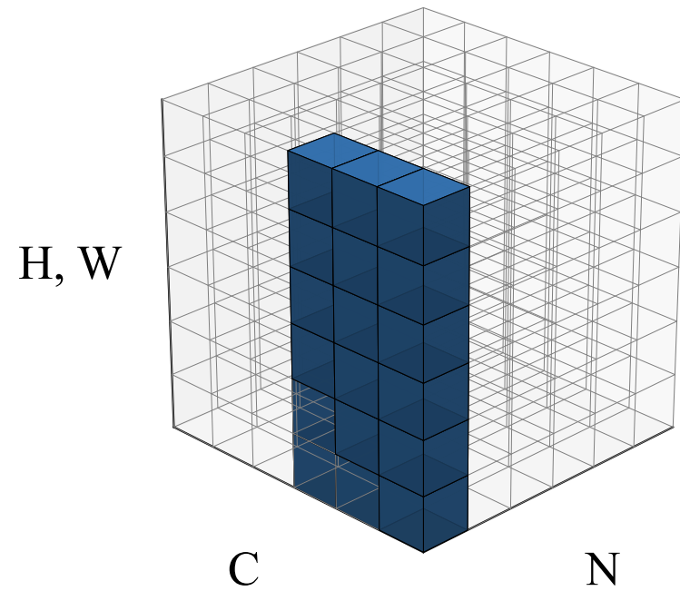
Group Norm
