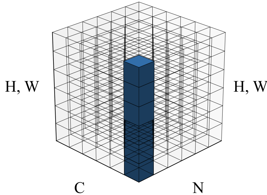
Instance Norm
