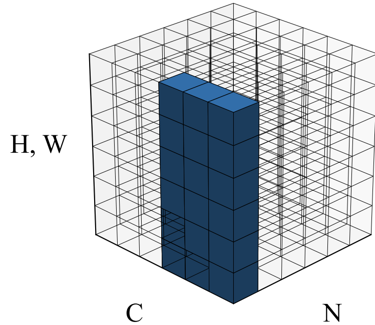
Group Norm
