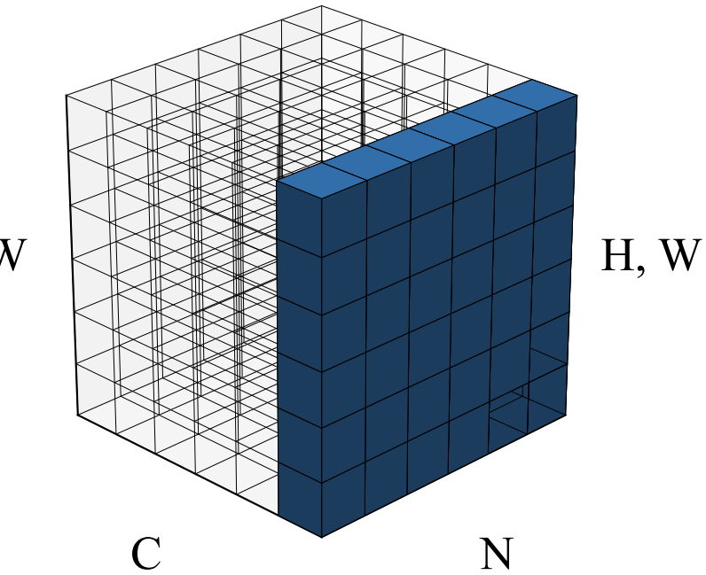
Batch Norm
