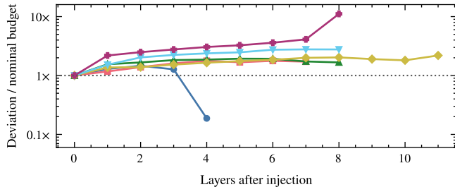
(a) Budget capped at injection only
