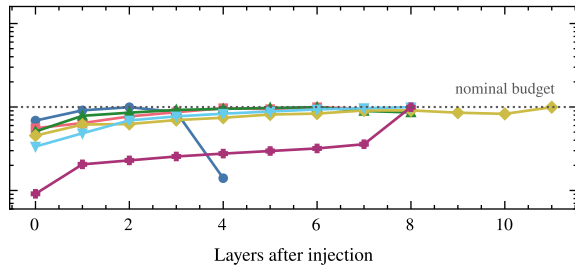
(b) Budget capped at every layer
