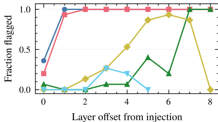
(c) Detection by depth · budget 0.0085
