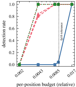
(b) GPT-2 layer 8: three read-outs
