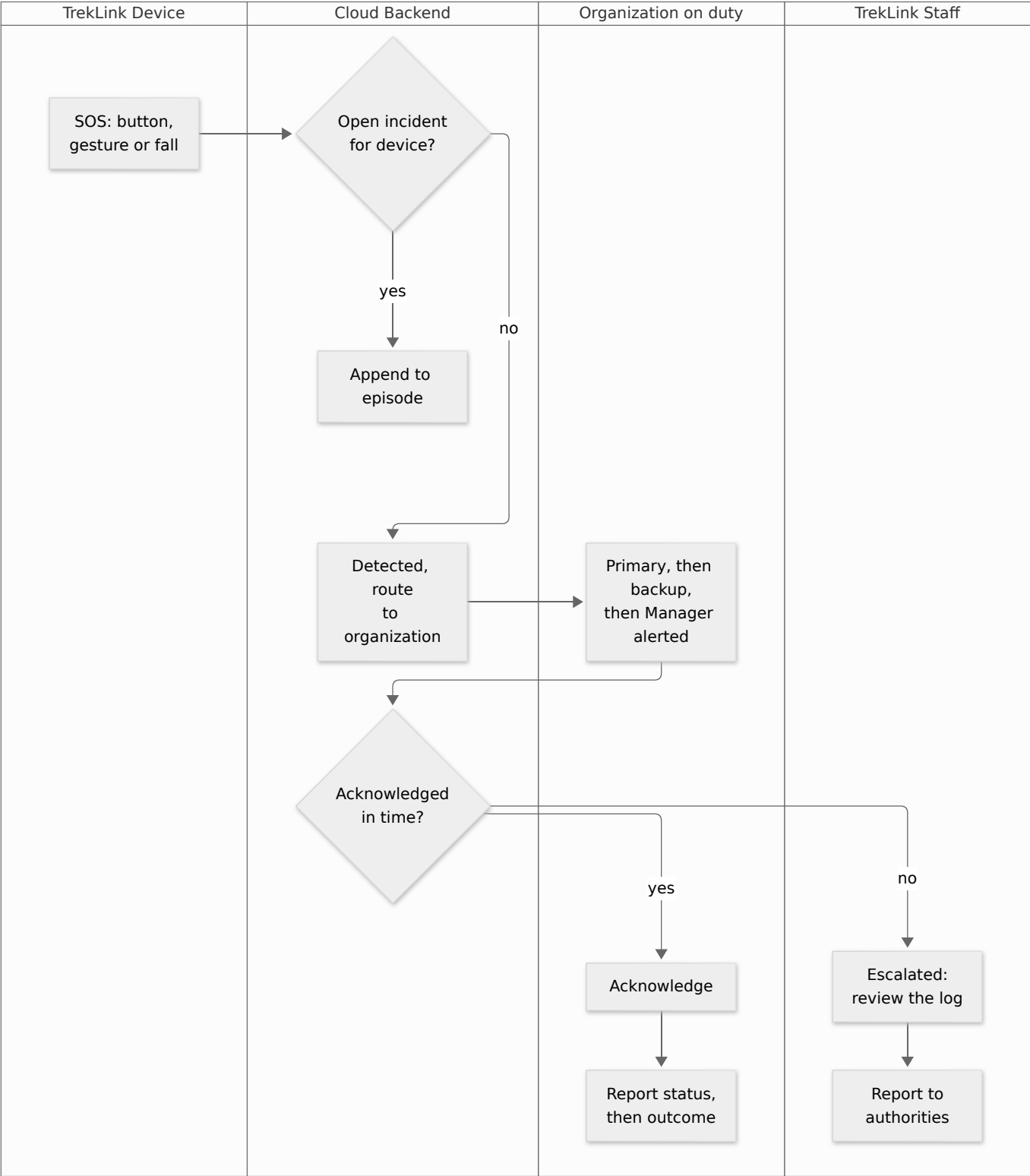
Figure 3: MF-03 SOS to Tiered alert to Escalation. Each tier has its own timeout; an unacknowledged alert always ends with TrekLink Staff. Placement: inline, 182.0 x 207.2 mm, labels at 7.71 pt.
