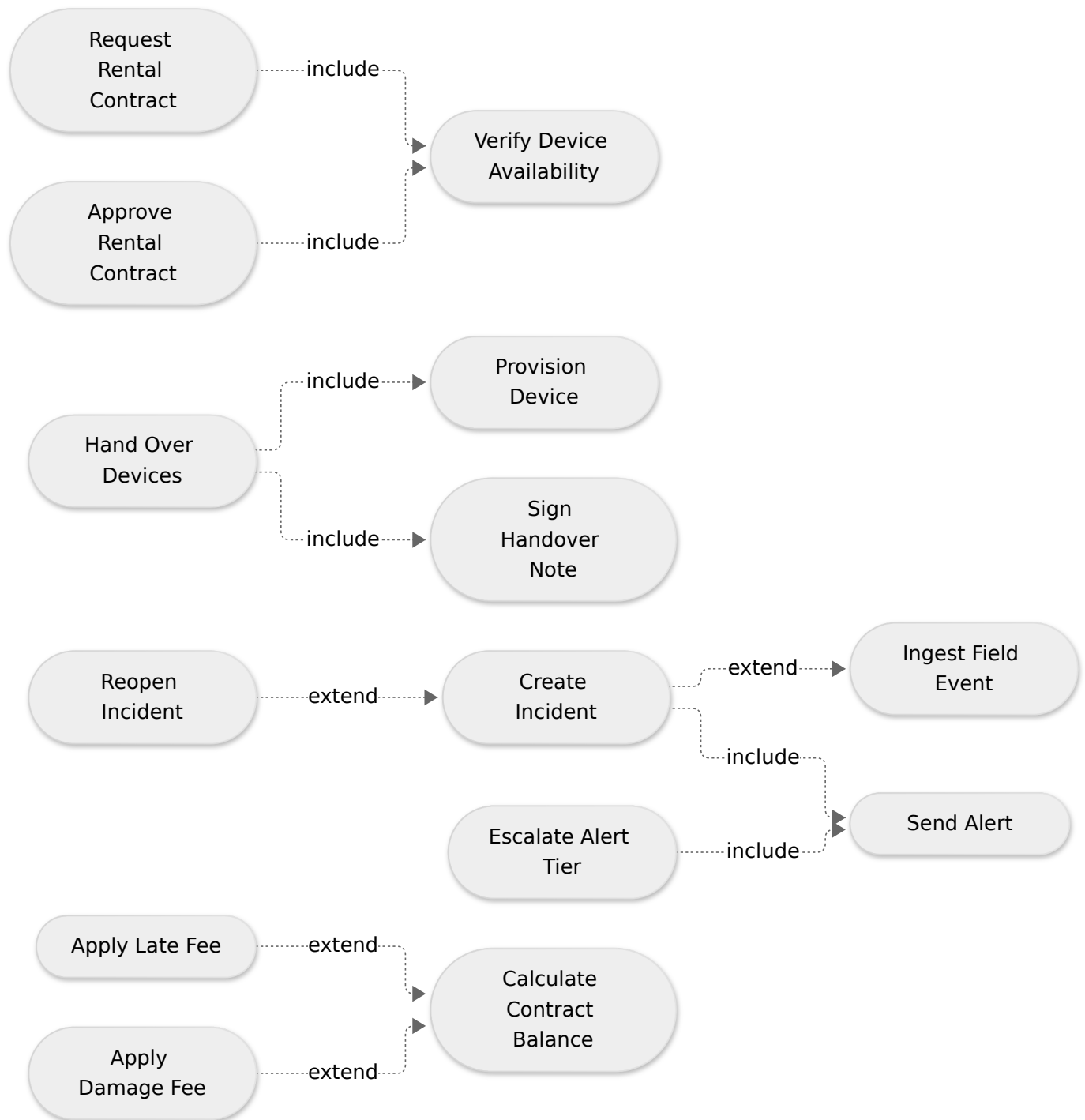
Figure 9: 'include' and 'extend' relationships. An included case always runs; an extending case runs only when its condition holds. Placement: rotated plate, 182.0 x 187.7 mm, labels at 10.21 pt.
