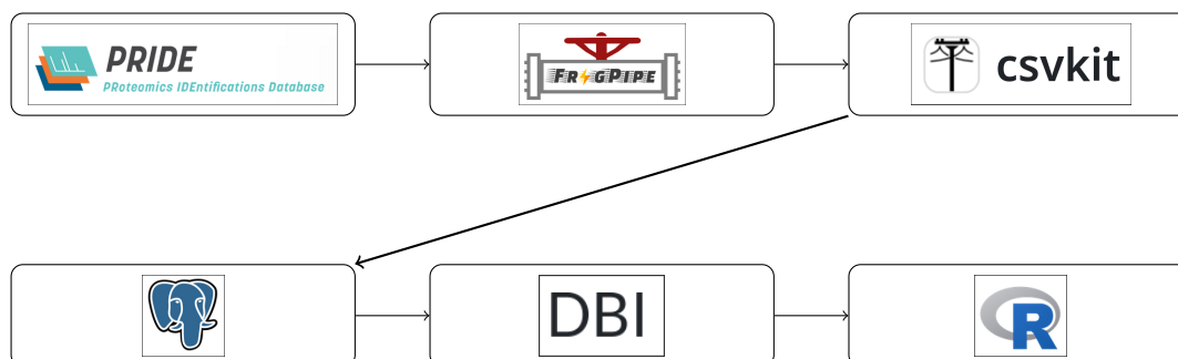
Figure 2: Overview of the workflow. Start by searching PRIDE for datasets. Run the datasets through FragPipe. Use csvkit to merge the outputs into a single table that can be used, and put into postgres. Use Postgres for data management and DBI to interact with it in R. Do the statistical work in R.
