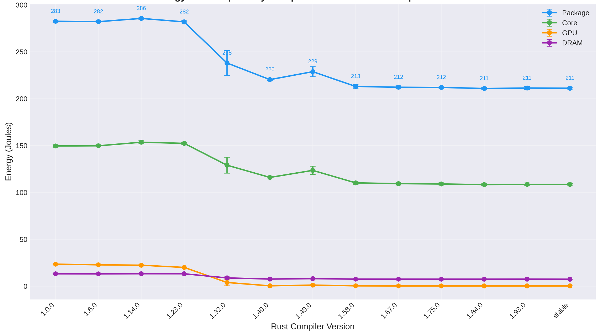
Energy Consumption by Component Across Rust Compiler Versions
